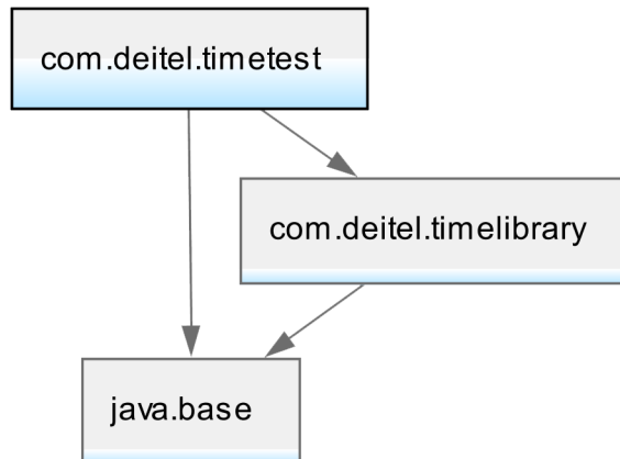
Fig. 36.15 | Module-dependency graph for the com.deitel.timetest module.
