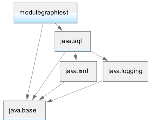
Fig. 36.16 | Dependency graph for a module that depends on java.sql .
