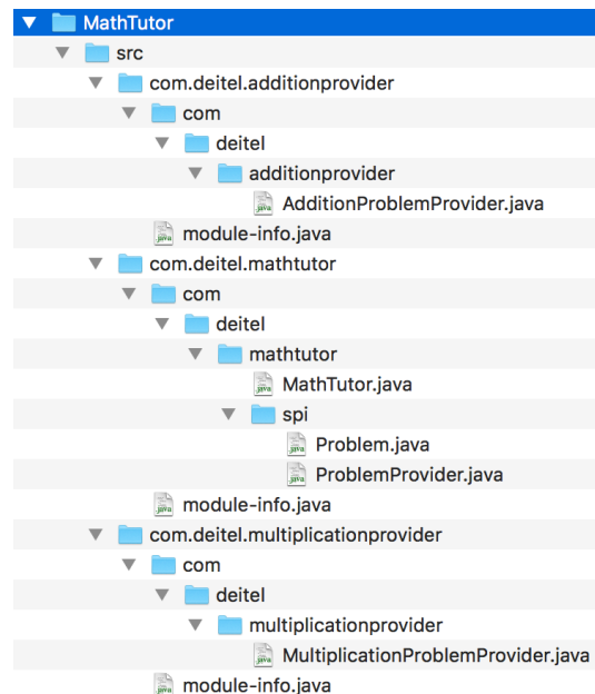
Fig. 36.25 | Folder structure for the MathTutor app's modules.
