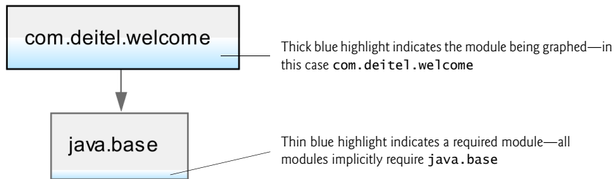
Fig. 36.8 | Module-dependency graph for the com.deitel.welcome module.
