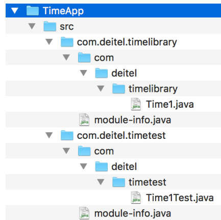
Fig. 36.10 | TimeApp example's src folder structure.
