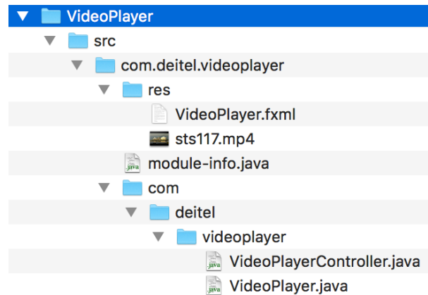
Fig. 36.20 | Modularized VideoPlayer src folder structure.
