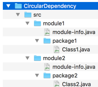
Fig. 36.18 | CircularDependency example's src folder structure.
